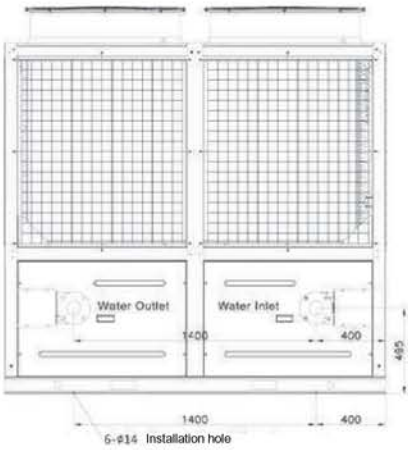
30RAM401XC 30RHM301/401XH
