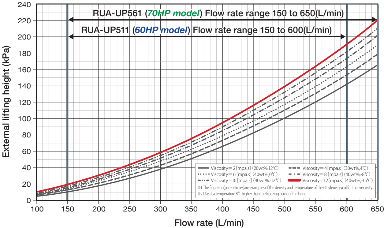
Internal resistance curve during brine use (pumpless model, ethylene glycol)
