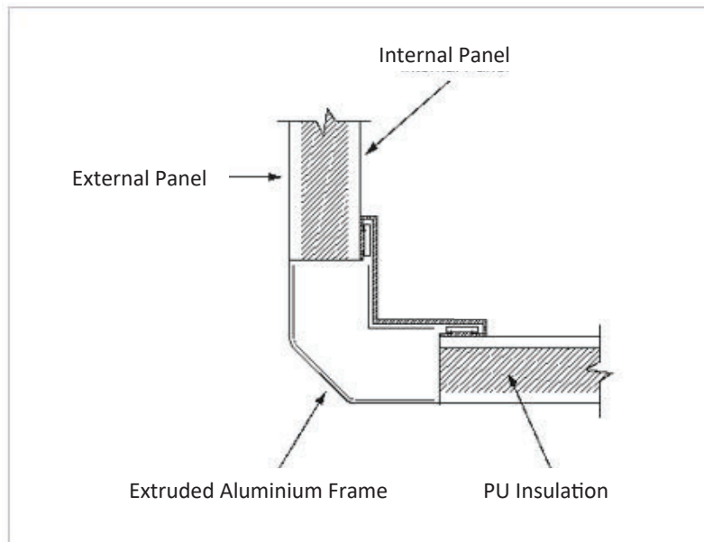
▲ Figure 4 Cross Section of Panel and Framework
