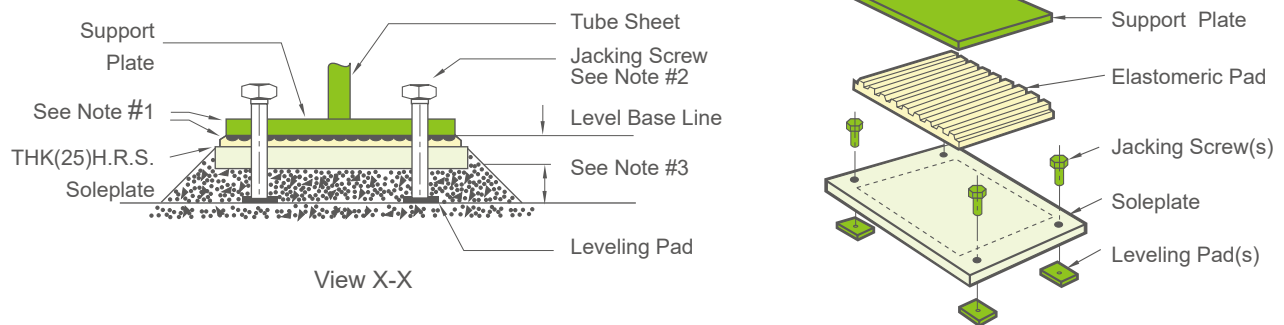
Rubber Isolation
